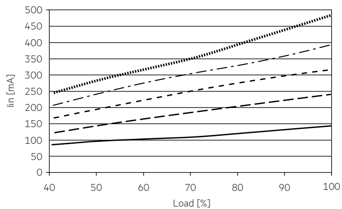
4.4.2 Input current vs. load 230 V, 50 Hz
