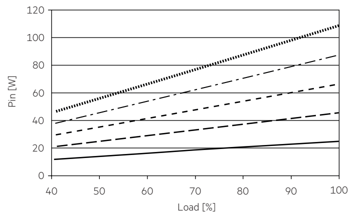
4.5.2 Input power vs. load 230 V, 50 Hz
